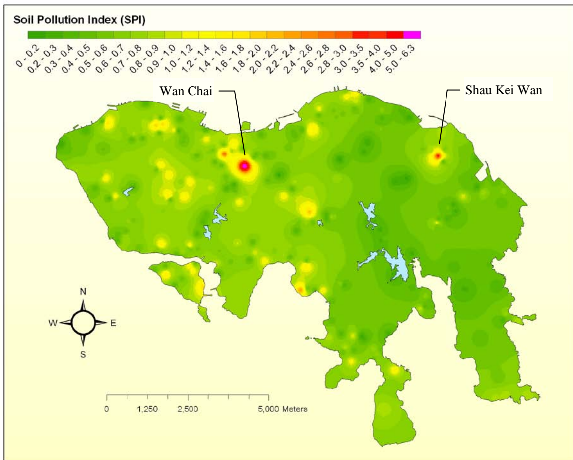
Fig. 6. Map of the Soil Pollution Index
