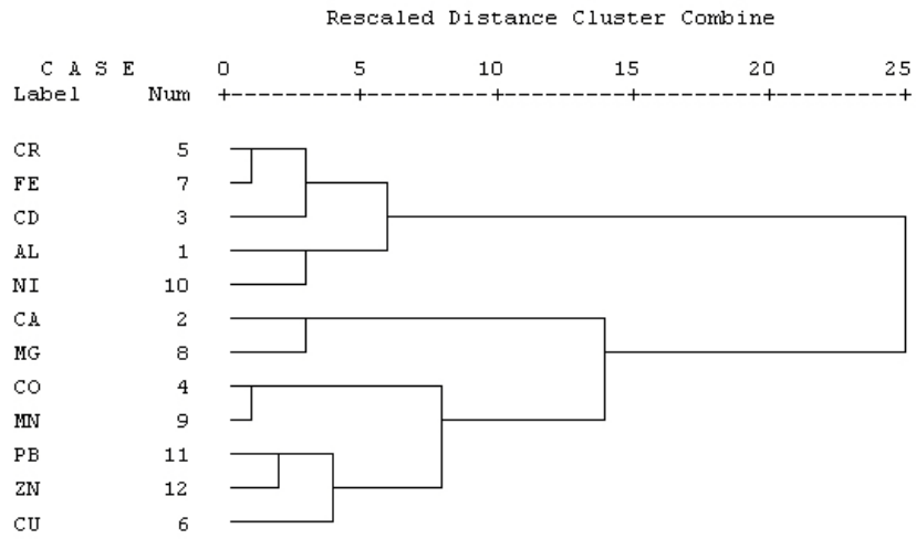
Fig. 4. Dendrogram of the cluster analysis of the country park soils based on their total concentrations (n=31)
