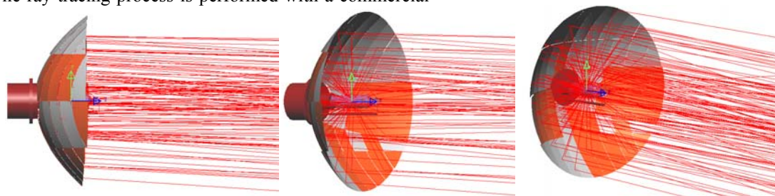
Fig. 4 Ray tracing
