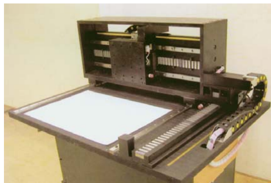
Fig.1 Cassette Type Motor
