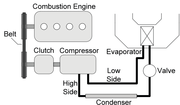
Fig.1: Basic structure of traditional automobile air conditioning system
