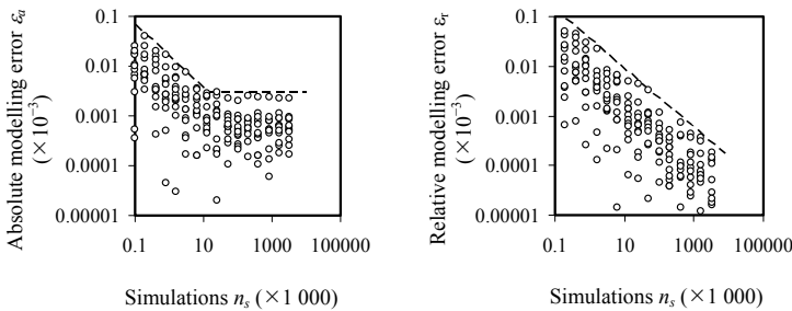
Figure 7 Stochastic model errors \varepsilon_a and \varepsilon_r versus simulation runs
