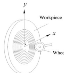
Figure 1. Kinematic configuration of ultra-precision spindle grinding
