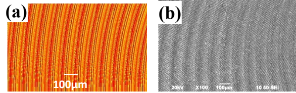
Figure 4. Comparison between simulation results (figure 4a) and experimental results (figure 4b) for surface generation in grinding. The scales of figure (a) and figure (b) are both 1000 \mu\text{m} \times 1000 \mu\text{m} .
