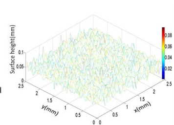
Figure 2. Simulated grinding wheel topography
