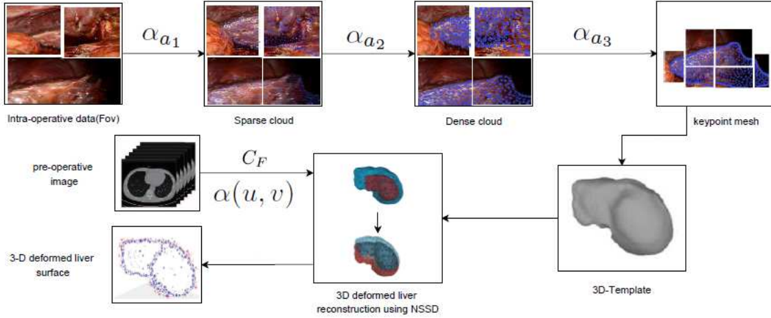
Fig. 2: Modeling a 3D template. From left to right: With intra-operative FOVs having functions of sparse cloud \alpha_{a1} , dense cloud \alpha_{a2} , and keypoint mesh \alpha_{a3} to reconstruct 3D template using mapping function, matching points and detected corners. Correspondence function C_F with \alpha(u, v) albedo of the liver surface maps deformation between the template and the pre-operative image using transformation F to reconstruct the deformed liver surface.
