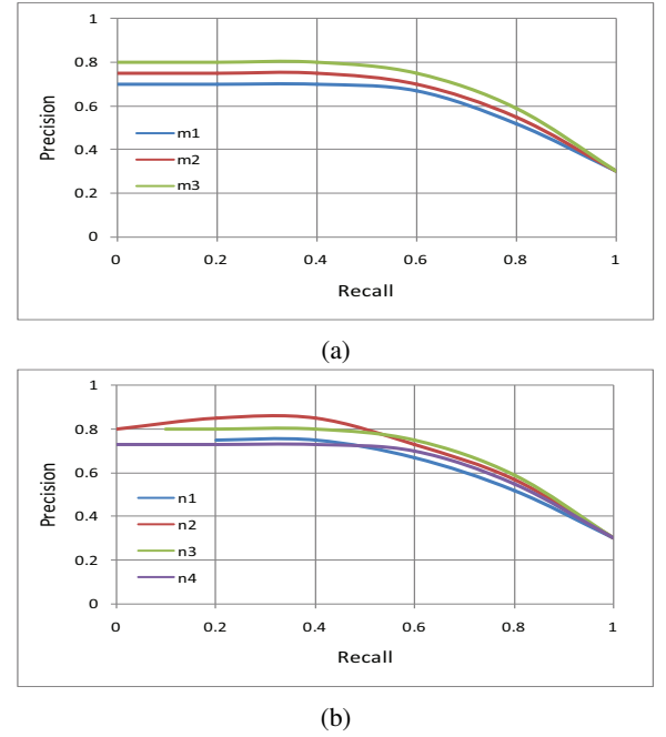
Fig. 8: Receiver operating characteristic (ROC) curve for estimating various affects of motion and noise on reconstruction results. (a) ROC for various degrees of motion m1 , m2 and m3 showing precision plotted against recall with area under the curve (AUC) maximum for m3 at 0.7944. (b) ROC for different levels of noise n1 , n2 , n3 and n4 for estimating affects of noise on our proposed model.
