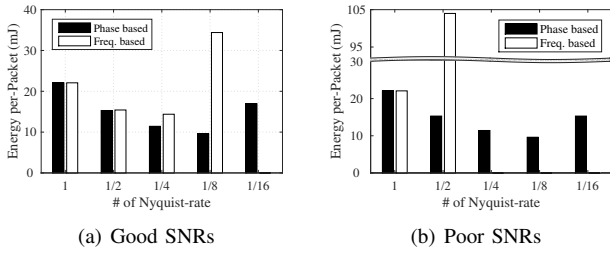
Fig. 17. Per-packet energy consumption under different downclocking factors. For the frequency-based approach, since no packets are correctly received in the cases of D=16 in good SNRs and D=4, 8, 16 in poor SNRs (see Fig. 14), the corresponding results are absent.
