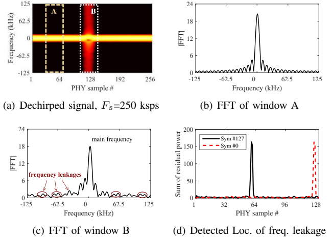
Fig. 7. Frequency-based fingerprint detection: (a) Dechirping the received chirp signal of Fig.4(b); (b,c) FFT results of the signal in window A and B; and (d) Frequency leakages detected from the under-sampled chirps of symbol #0 and #127, ambiguity symbols have different fingerprints.
