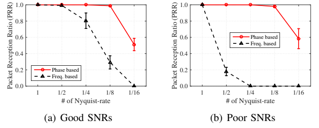
Fig. 14. Impacts of downclocking on Packet Reception Ratio (PRR).
