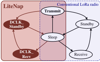
Fig. 10. State transitions of LiteNap .
