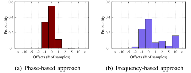
Fig. 13. Histogram of offsets (in # of PHY samples) between the extracted fingerprints and the ideal locations under the downclocking factor of D=8 .
