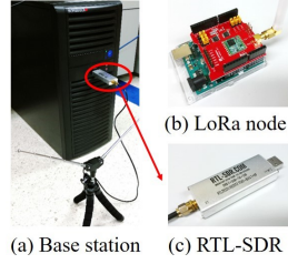
Fig. 11. Experiment devices.
