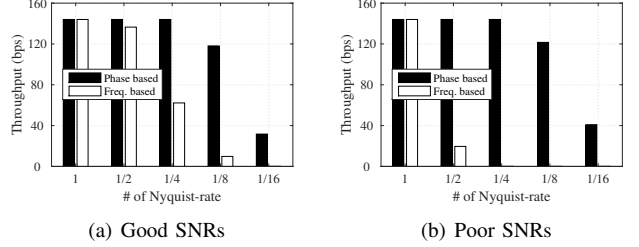
Fig. 15. Impacts of downclocking on throughput.
