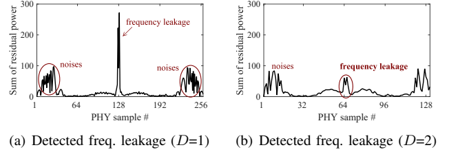
Fig. 8. Impacts of noise on the detection of frequency leakage: Detecting results of (a) fully-sampled and (b) under-sampled chirps. Frequency leakage is buried within noise in the case of down-sampling (e.g., D=2 ).
