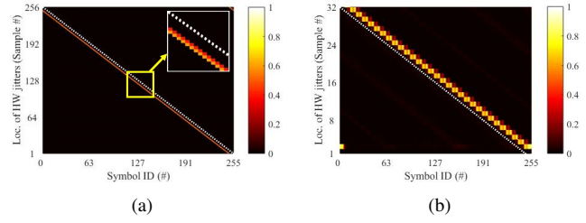
Fig. 12. The fingerprints of all 256 symbols extracted from (a) fully-sampled chirps and (b) under-sampled chirps (downclocking factor D=8 ), respectively.
