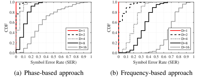
Fig. 16. Performance of downclocked symbol demodulation in good SNRs.
