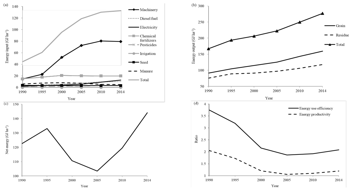
Fig. 2: Energy indicators for crop production in Anhui Province during 1990-2014.
