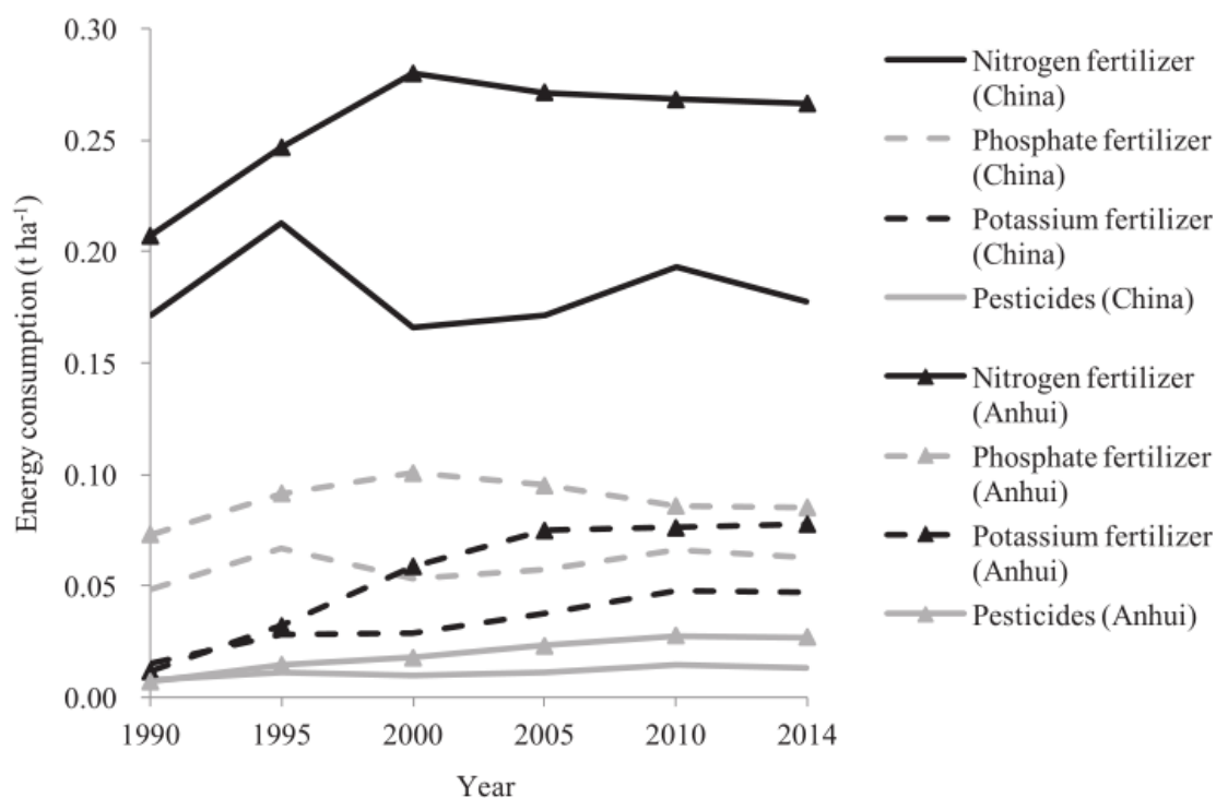
Fig. 6: Comparisons of energy consumptions from crop production between China and Anhui Province during 1990-2014.
