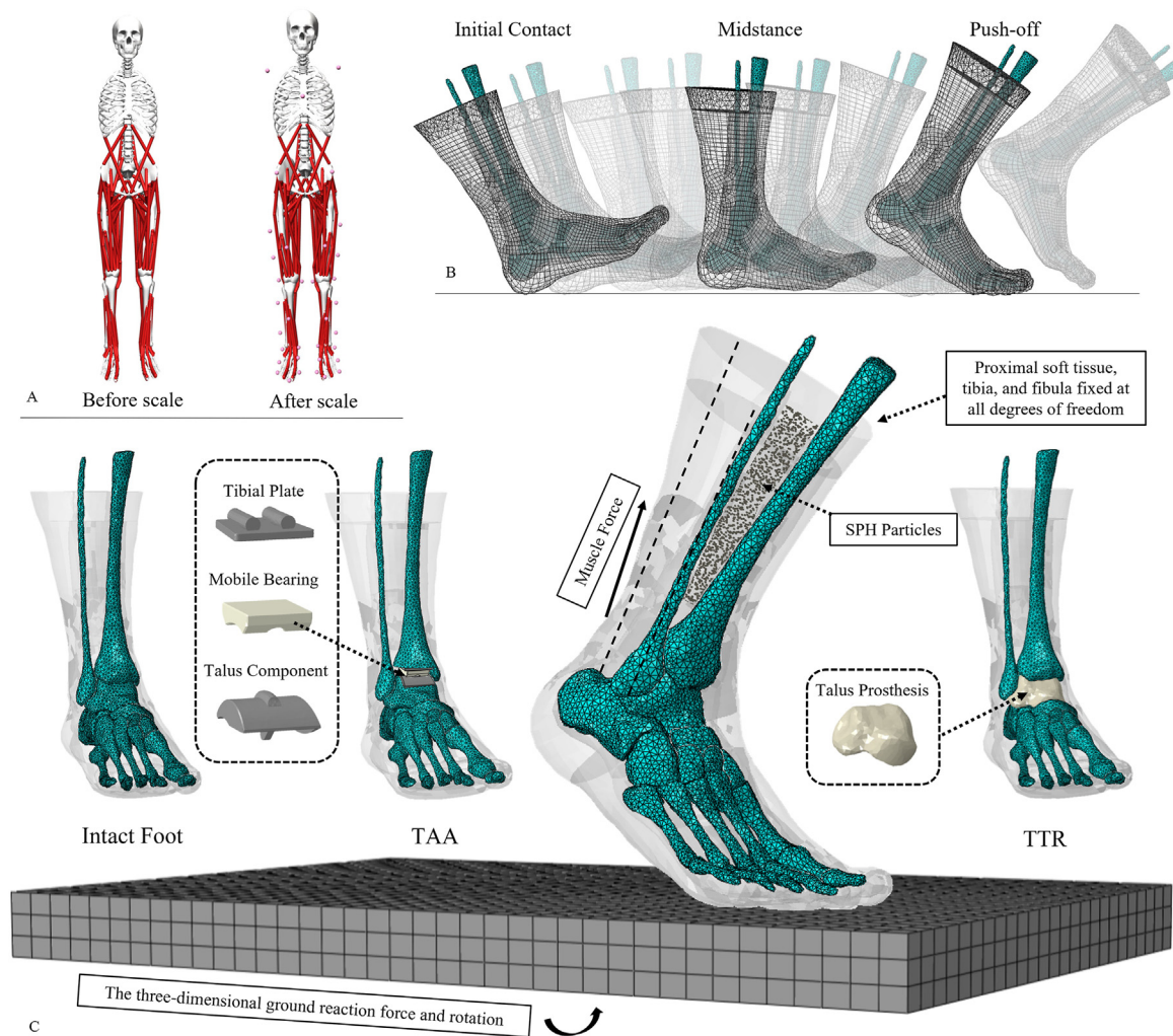
Fig. 1. A) Subject-specific scaling of the musculoskeletal model; B) Simulation of the walking gait; C) Configurations of the three models and loading/boundary conditions for the finite element analyses. SPH: smoothed-particle hydrodynamics; TTR: total talus replacement; TAA: total ankle arthroplasty.
