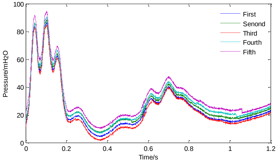
Figure 5 | Measured transient pressure traces at S1
