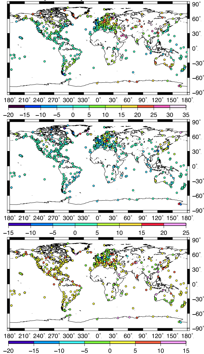
Figure 7 Relative WRMS reductions obtained when correcting ITRF2014 residual time series from MERRA-2-derived ATML displacements for all 596 stations. Unit is %
