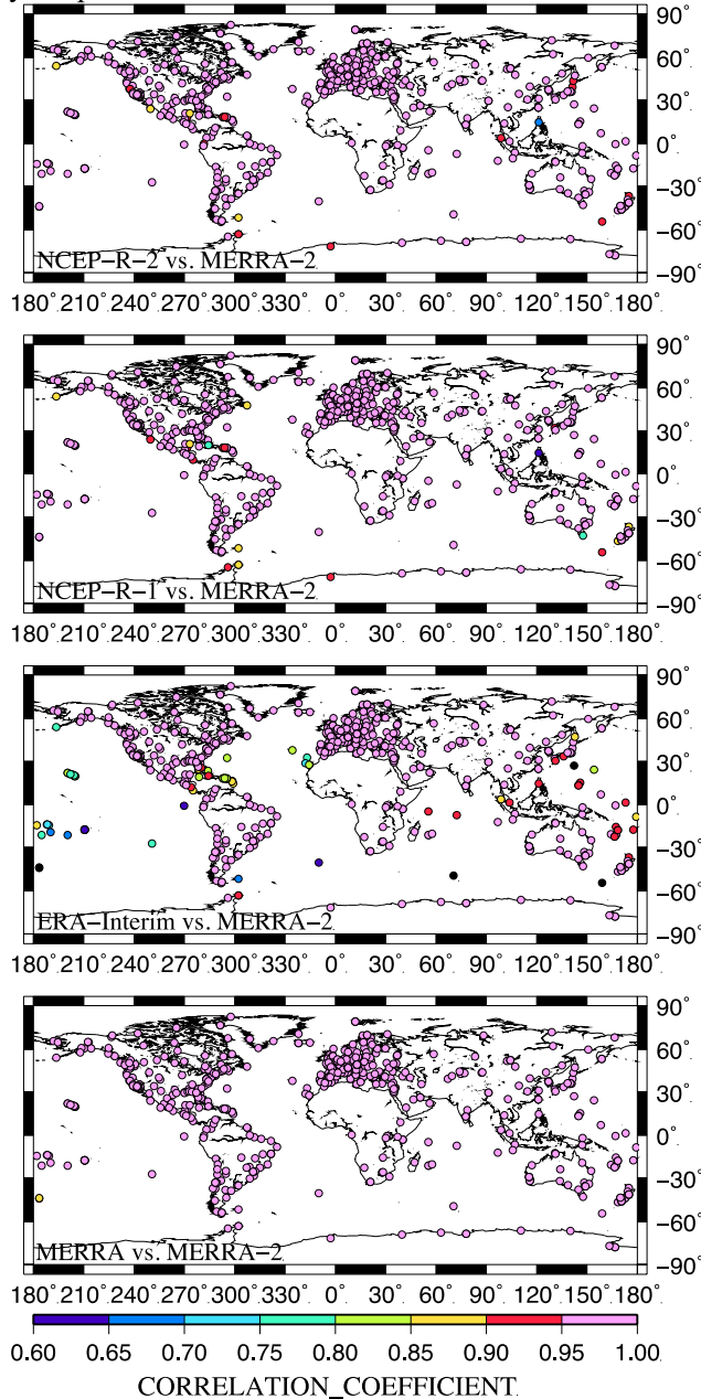
Figure 9 Correlation coefficients for the Up component between ATML displacements derived from MERRA-2 and the other 4 SP datasets for all 596 stations. Black dots indicate the correlation coefficients are smaller than the minimum value of the scale
