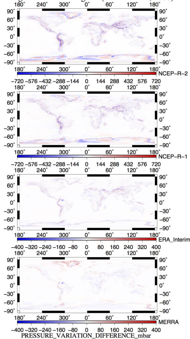
Figure 12 Daily pressure variation differences of the four SP models w.r.t MERRA-2 on 2014.07.15. Unit of the pressure variation difference is mbar. From top to bottom panels represent the NCEP-R-2, NCEP-R-1, ERA-Interim and MERRA product.
