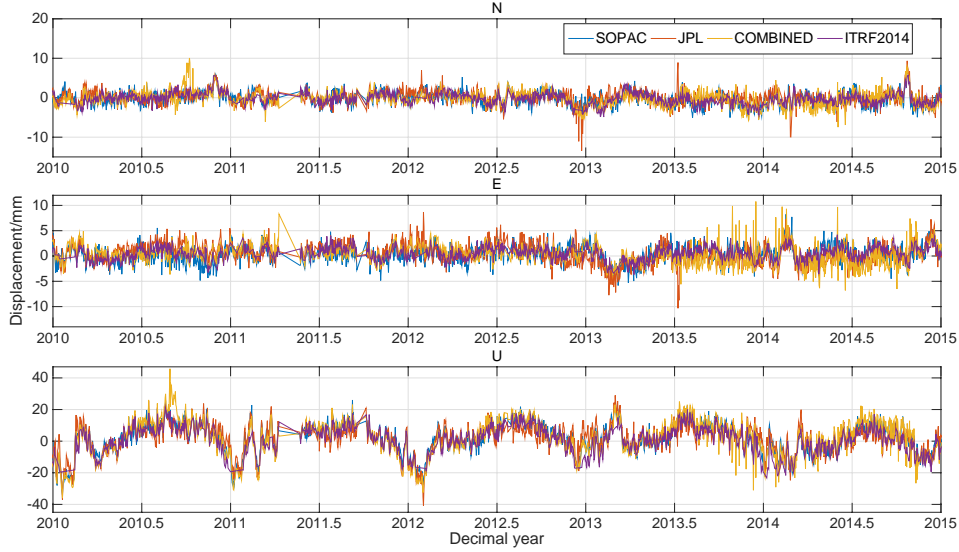
Figure 1 Cleaned residual time series for station ARTU from different institutions. The blue curve represents the product from SOPAC, red indicates the JPL solution, orange illustrates the combined solution from SOPAC and JPL, while purple demonstrates the ITRF2014 residuals.
