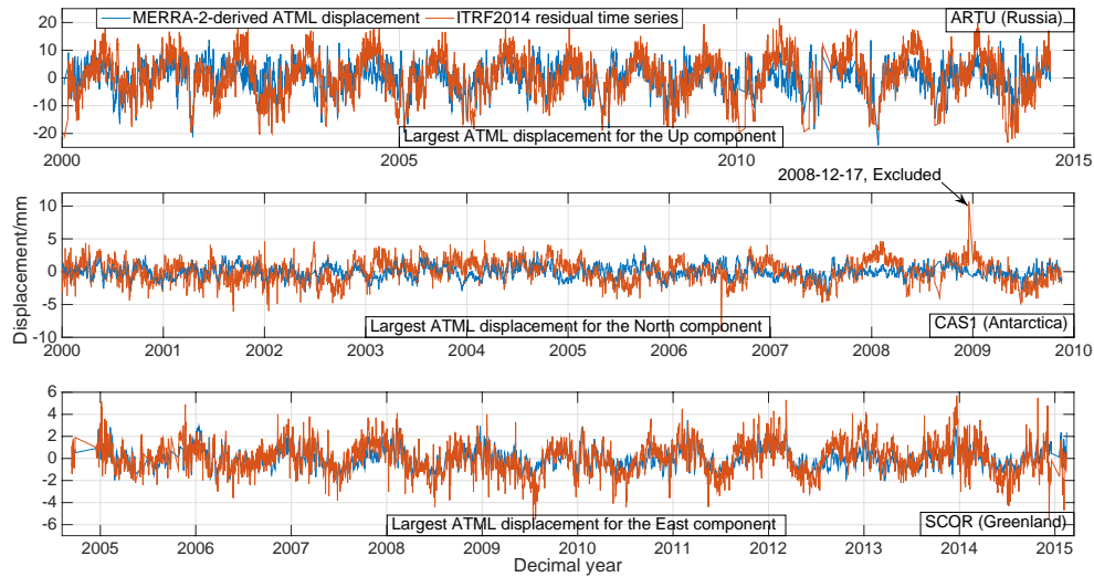
Figure 3 Time series of stations with maximum MERRA-2-derived ATML displacement (blue curve) together with their corresponding ITRF2014 residuals (red curve)
