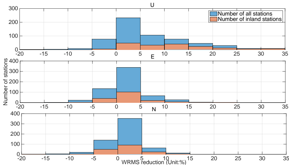
Figure 8 Histogram of relative WRMS reduction. The X label describes the WRMS reduction (Unit: %). The Y label illustrates the number of stations with WRMS reduction inside different ranges. Blue color represents the results for all 596 stations, while orange denotes the 174 inland stations
