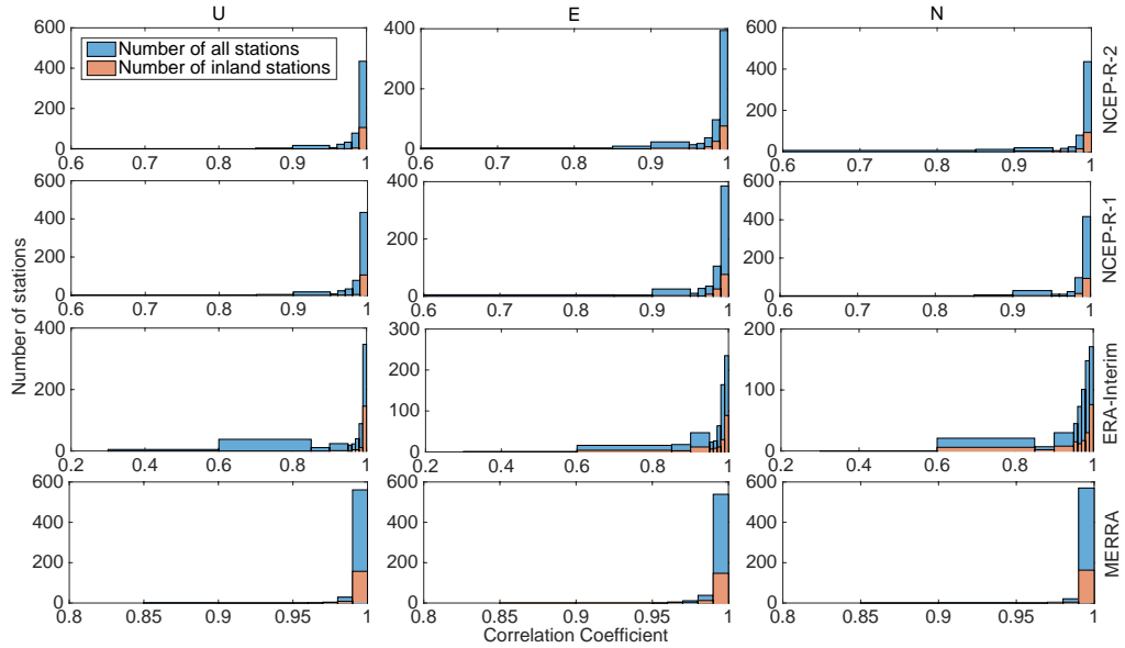
Figure 10 Histogram of correlation coefficient between MERRA-2 and other model derived ATML displacement for the Up, East and North components. The X label describes the correlation coefficient. The Y label illustrates the number of stations with correlation coefficient inside different ranges. Blue color represents the results for all 596 stations, while orange denotes the results for inland stations
