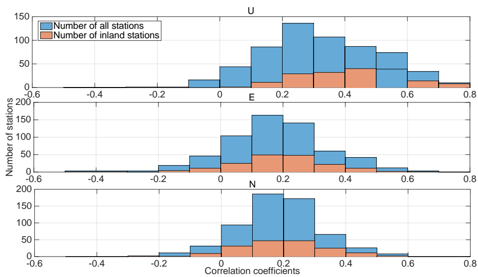
Figure 6 Histogram of correlation coefficients between MERRA-2-derived ATML displacements and the ITRF2014 residual time series. The X label describes the correlation coefficient. The Y label illustrates the number of stations with correlation inside different ranges. Blue color represents the results for all 596 stations, while
