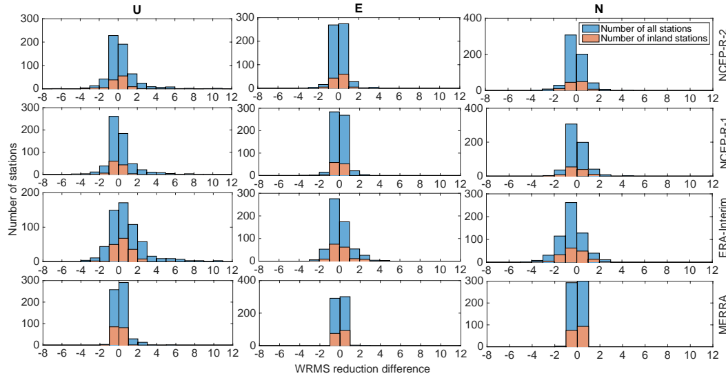
Figure 11b Histogram of relative WRMS reduction differences (%) of different models w.r.t MERRA-2 for the Up (U), East (E) and North (N) components. The X label describes the WRMS reduction difference. The Y label illustrates the number of stations with WRMS reduction difference inside different ranges. Blue color represents the results for all 596 stations, while orange denotes the results for inland stations
