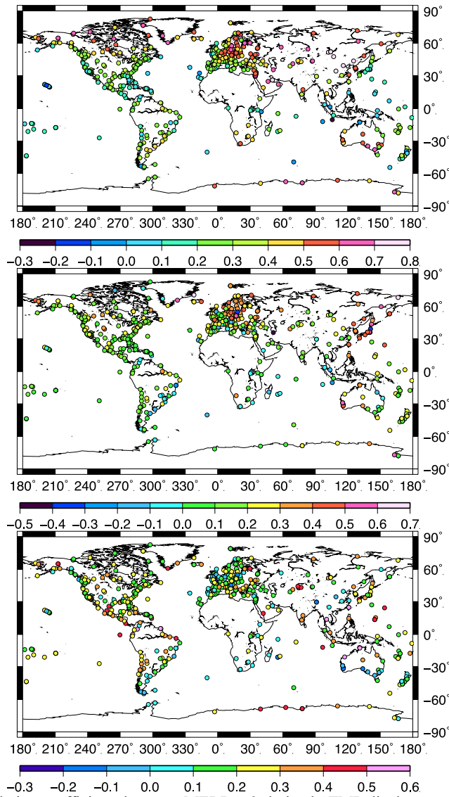
Figure 5 Correlation coefficients between MERRA-2-derived ATML displacements and the ITRF2014 residual time series for all 596 stations.
