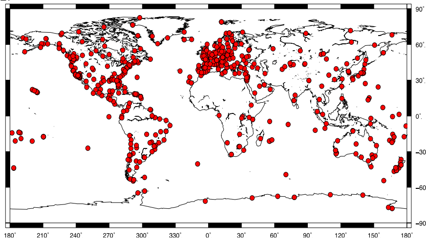
Figure 2 Spatial distribution of the 596 selected GNSS stations
