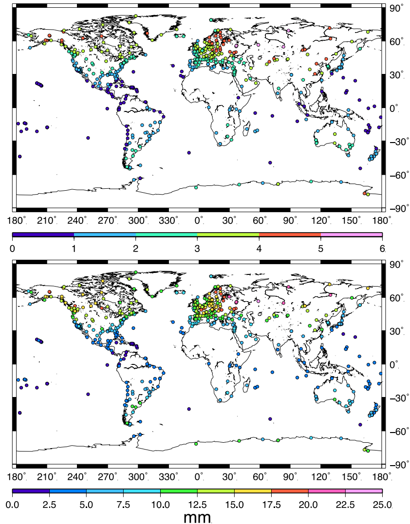
Figure 4 RMS (top) and maximum amplitudes (bottom) of the 6-hourly MERRA-2-derived ATML displacement time series for the Up component. Units are mm.
