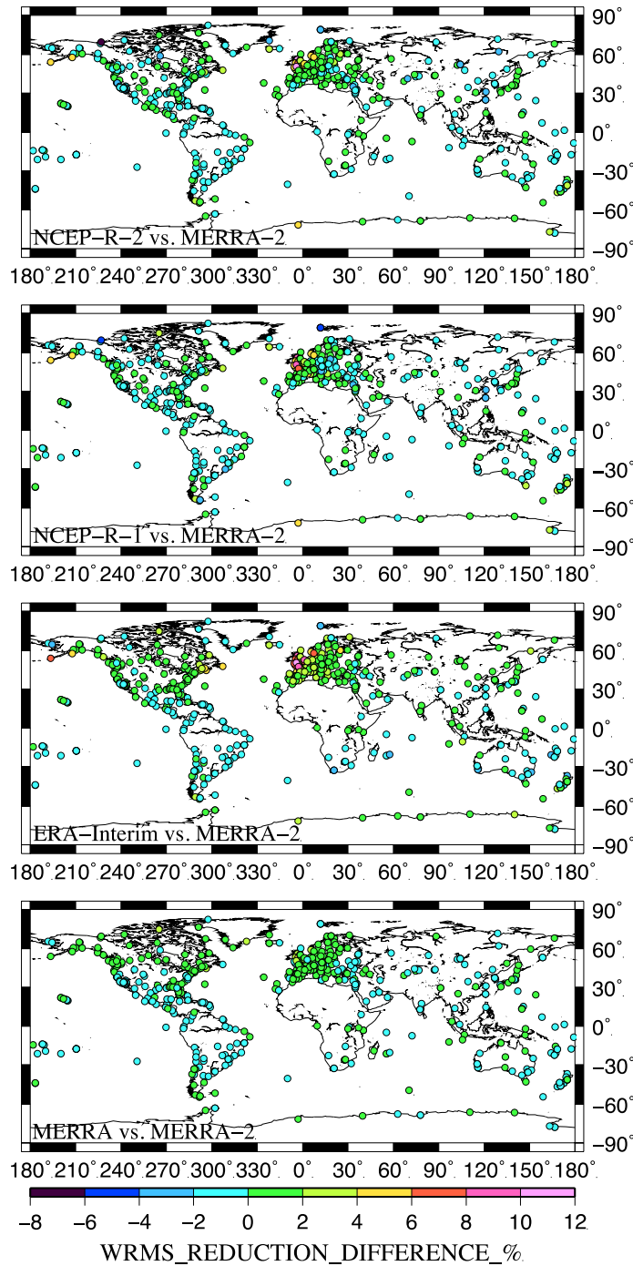
Figure 11a Relative WRMS reduction differences (%) of different models w.r.t MERRA-2 for the Up component of all 596 stations.
