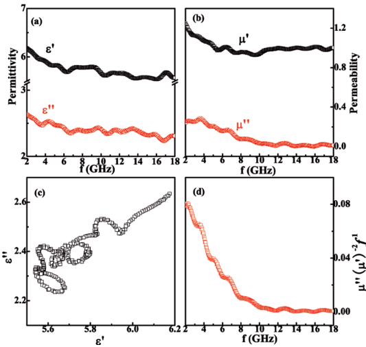
Figure 3: (a) Complex permittivity and (b) permeability, (c) Cole-Cole semicircles and (d) values of \mu''(\mu')^{-2}f^{-1} as a function of frequency for the composite with 40 wt% NiFe 2 O 4 nanosheets.
