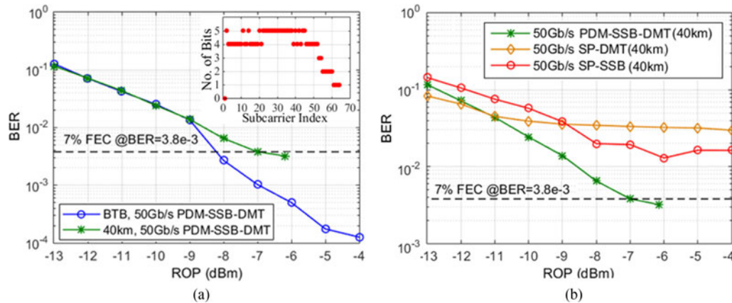
Fig. 12. BER performance as a function of the recovered optical power (a) 50 Gb/s PDM-SSB-DMT with BTB and 40 km SSMF transmissions, (b) different system schemes for 40 km SSMF transmission.
